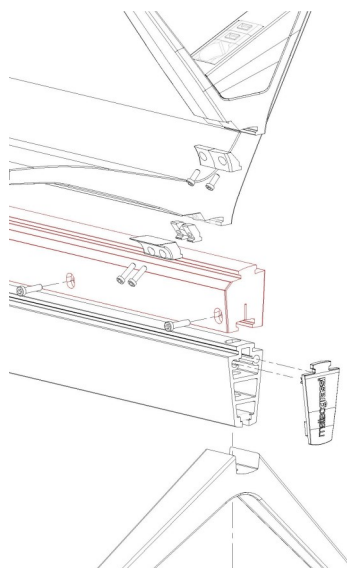
Special Seat Support for ADA Seat
